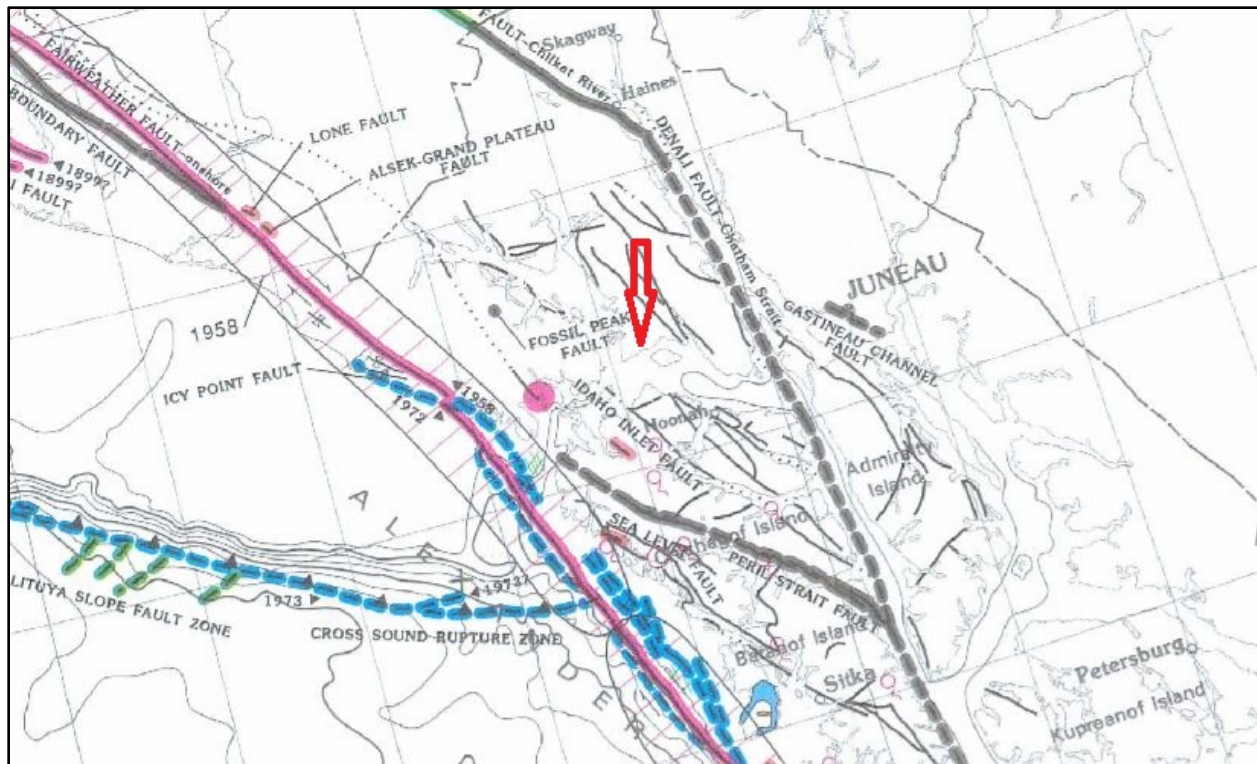
Figure 4. Alaska's Neotectonic Map of Alaska, Gustavus Area
