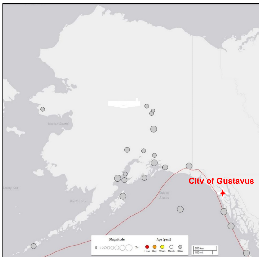
Figure 6. City of Gustavus Earthquake Probability
